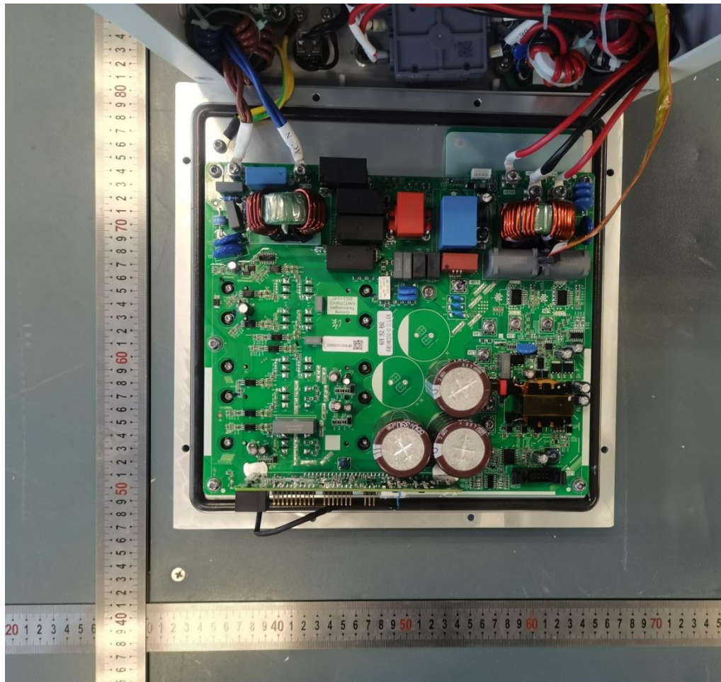
Internal view
